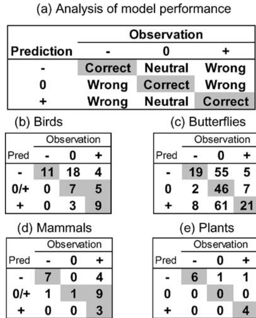
Figure 5 Analysis of the performance of the edge effect model (Figure 4). (a) Outcomes are separated into cases in which the model was correct and incorrect. Incorrect outcomes are further separated into two separate cases in which an unpredicted neutral response was observed and cases in which wrong positive or negative responses were observed. Results are presented for tests of the model on four taxa. (b) Bird results are from Ries & Sisk (2004). (c) Butterfly results are from Ries (2003). (d) Mammal and (e) plant results are from a review of the literature, and details for these tallies are given in Appendix 1b. (The Appendix is included as Supplemental Material. Follow the Supplemental Material link from the Annual Reviews home page at http://www.annualreviews.org .) Note that for birds and mammals, we lacked information to differentiate between positive and neutral predictions in some cases, so outcomes were identified as correct if either observation was recorded. Outcomes for which model predictions were correct are shaded in gray.
